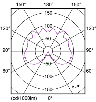
Light Distribution Diagram - 5.5A15/LED/827-22/E12/CL/DIM 120V
