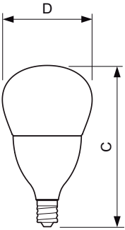
SS Candle A15 120V 5W-40W 300lm E12 D
