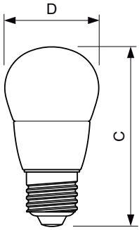
SS Clear Bulb A15 CL 6W-40W 450lm 330D E26D
