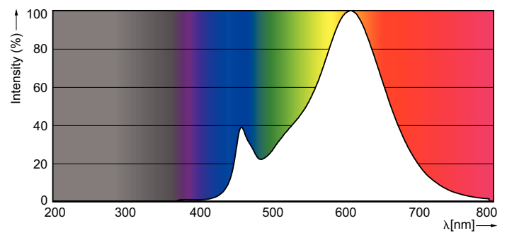
LED Bulb 6-40W A15 E26 CL
