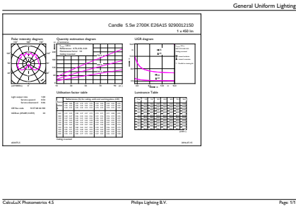
General uniform lighting - 5.5A15/LED/827-22/E26/CL/DIM 120V
