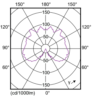
Light Distribution Diagram - 5.5A15/LED/827-22/E26/CL/DIM 120V
