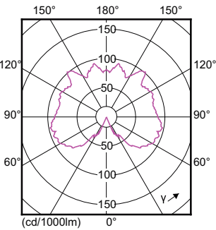
Light Distribution Diagram - 6A19/LED/827-22/CL/DIM 120V
