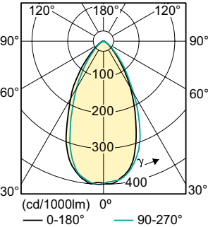
Light Distribution Diagram - MAS LEDspotMV VLE D 4.3-50W GU10 827 60D
