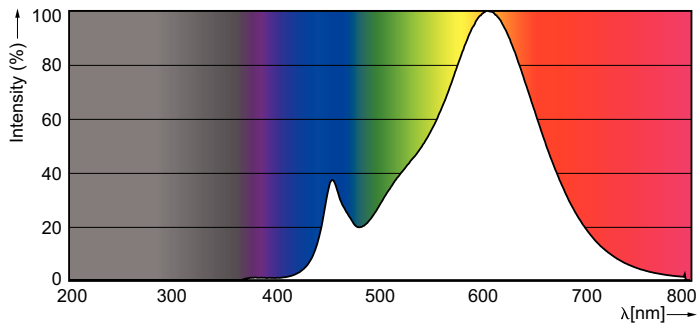
LED Lamps, CorePro LEDspotMV 3.5-35W GU10 PAR16 827 255lm 36D
