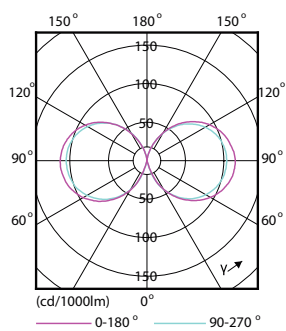
Light Distribution Diagram - 40ED28/LED/730/ND 120-277V 4/1
