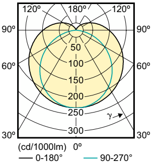
Light Distribution Diagram - 16.5T8 LED/48-4000 IF 10/1 UHO
