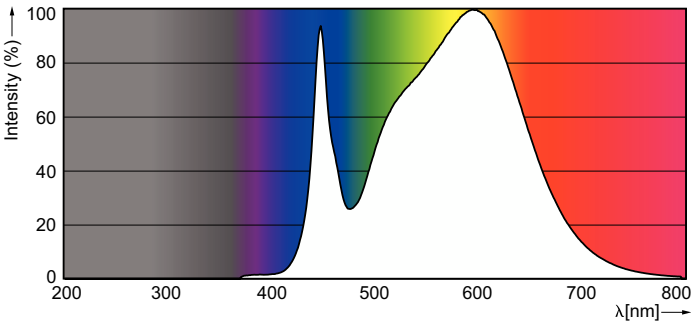
Spectral Power Distribution Colour - 16.5T8 LED/48-4000 IF 10/1 UHO
