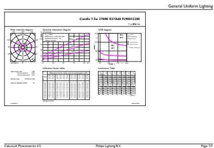
Classic LEDBulb D 7.5-60W A60 827 CL
