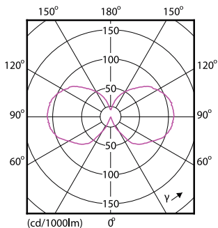
Classic LEDBulb D 7.5-60W A60 827 CL
