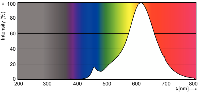
Spectral Power Distribution Colour - LEDClassic 50W G120 E27 2000K GOLD D
