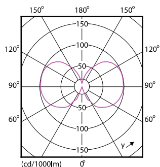
Light Distribution Diagram - LEDClassic 50W G120 E27 2000K GOLD D
