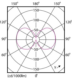
Light Distribution Diagram - LEDClassic 50W G120 E27 2000K GOLD D
