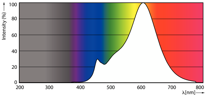
Spectral Power Distribution Colour - LED Globe 60W G93 E27 WW FR ND 1CT/4
