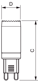
Capsule 230V 2.3W-25W 210lm 2700K G9 D
