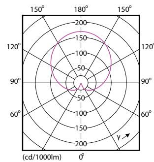
MAS LEDbulb DT 6-40W A60 E27 FR
