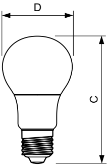
Entry bulb 6.5W-45W 470lm150D 2700K E27D
