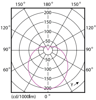
Light Distribution Diagram - LED SSW 60W A60 E27 WW FR ND RF 1BC/6
