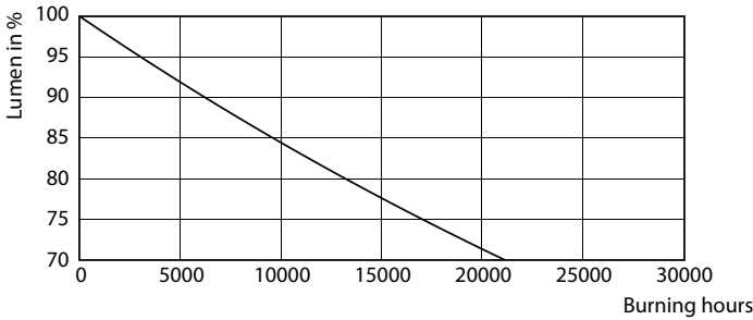
Lumen Maintenance Diagram - LED SSW 60W A60 E27 WW FR ND RF 1BC/6
