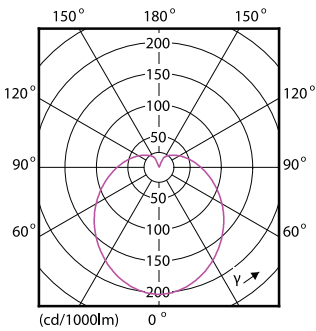
Light Distribution Diagram - LED SSW 60W A60 E27 WW FR ND 1SRT4
