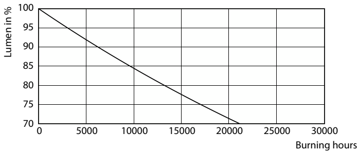
Lumen Maintenance Diagram - LED SSW 60W A60 E27 WW FR ND 1SRT4
