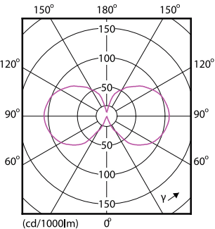
Light Distribution Diagram - LEDClassic 60W A60 E27 WW CL ND
