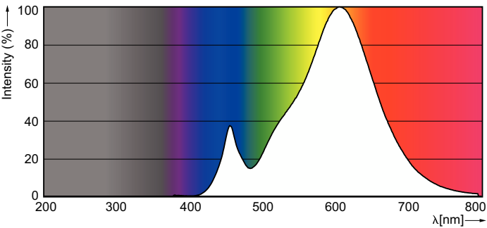
Spectral Power Distribution Colour - LEDClassic 60W A60 E27 WW CL ND
