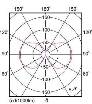
Light Distribution Diagram - CLA LEDBulb ND 4-40W ST64 E27 827 CL
