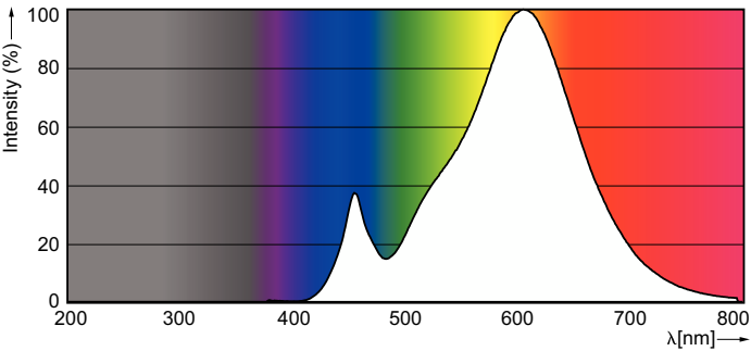
Spectral Power Distribution Colour - LEDClassic 4-50W ST64 E27 WW CL ND APR
