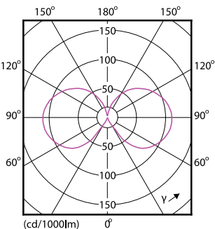
Light Distribution Diagram - LEDClassic 2-25W BA35 E14 WW CL ND APR
