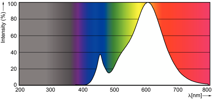
Spectral Power Distribution Colour - LEDClassic 60W G93 E27 WW CL ND
