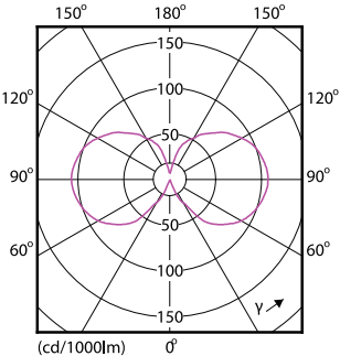
Light Distribution Diagram - LEDClassic 60W G93 E27 WW CL ND
