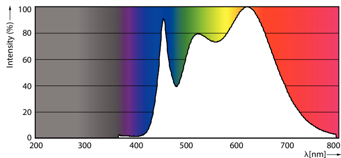
Spectral Power Distribution Colour - MAS LED MR16 ExpertColor 7.2-50W 940 24D
