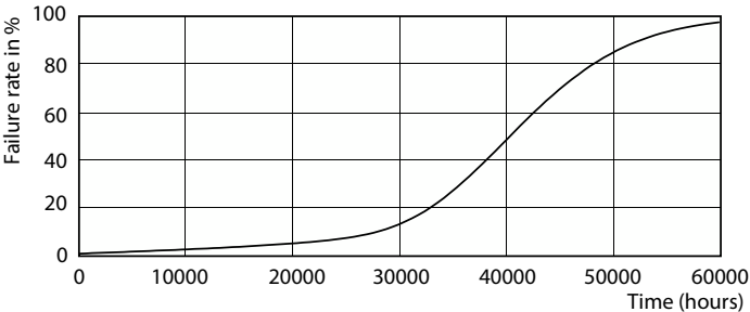
Life Expectancy Diagram - MAS LED MR16 ExpertColor 7.2-50W 927 36D
