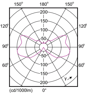
Light Distribution Diagram - CorePro LEDcapsuleLV 2-20W G4 827
