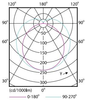
Light Distribution Diagram - MAS LEDtube 1200mm 16W865 T8 I
