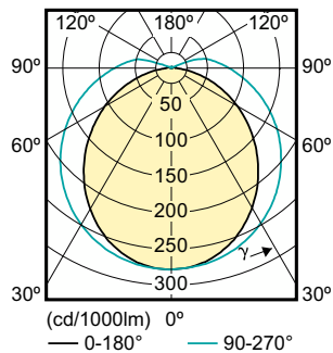
Light Distribution Diagram - LED 3W 300mm S14D WW ND 1CT/4
