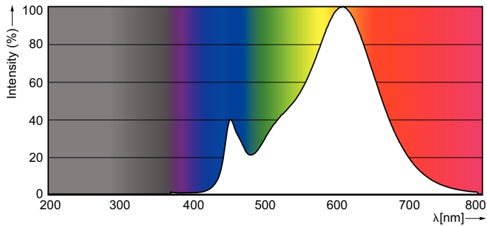
Spectral Power Distribution Colour - LED 3W 300mm S14D WW ND 1CT/4
