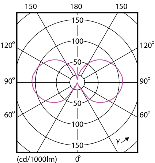
Light Distribution Diagram - LEDClassic 40W B35 E14 WW CL ND
