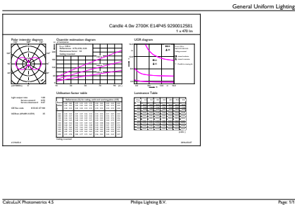
General uniform lighting - LEDClassic 40W P45 E27 WW CL ND
