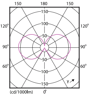
Light Distribution Diagram - LEDClassic 40W P45 E27 WW CL ND
