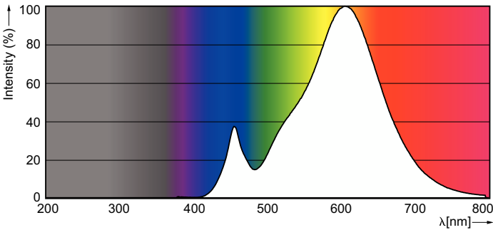
Spectral Power Distribution Colour - LEDClassic 40W P45 E27 WW CL ND
