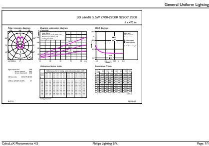
General uniform lighting - LED SSW 40W B38 E14 WW CL ND 2CT/4
