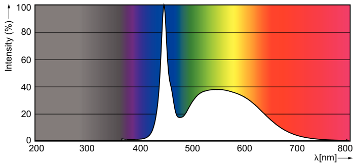
LED 1-25W B35 E14 865 200lm
