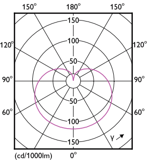
Light Distribution Diagram - BC9.5A19/AMB/827-50-22/ND SSCC 120V
