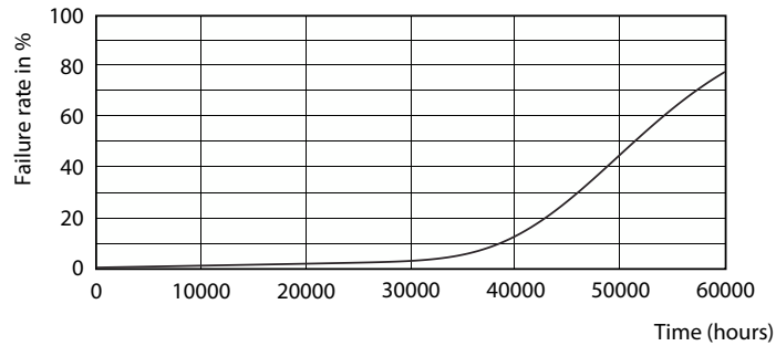
Life Expectancy Diagram - 165HB/LED/840/ND WB UDL 2/1
