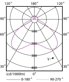
Light Distribution Diagram - 165HB/LED/840/ND WB UDL 2/1
