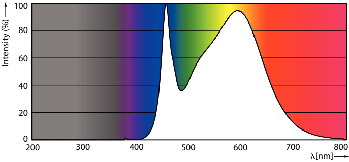
Spectral Power Distribution Colour - 165HB/LED/840/ND WB UDL 2/1
