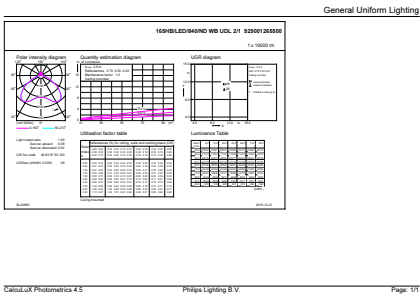
General uniform lighting - 165HB/LED/840/ND WB UDL 2/1
