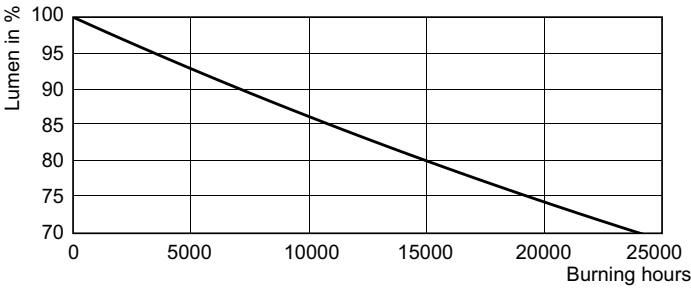
Lumen Maintenance Diagram - ESS LED MR16 4.5-50W 36D 830 100-240V
