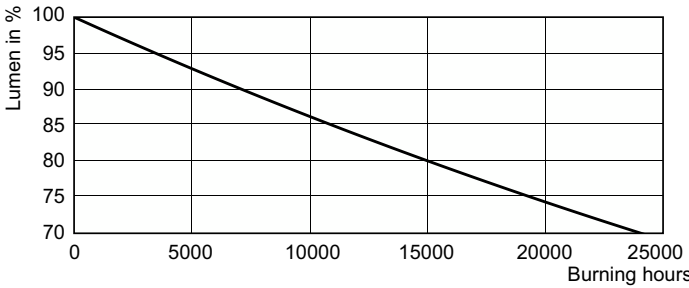
Lumen Maintenance Diagram - ESS LED MR16 4.5-50W 36D 865 100-240V
