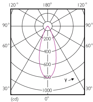
Light Distribution Diagram - ESS LED MR16 4.5-50W 36D 865 100-240V
