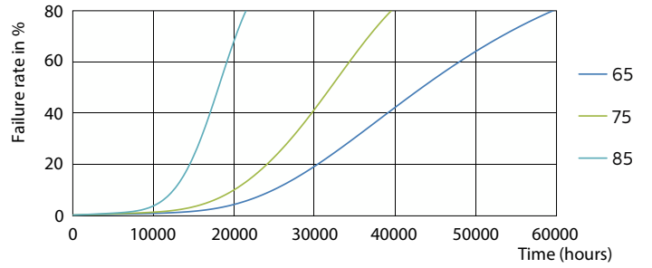
Life Expectancy Diagram - LED PLC 6.5W 865 2P G24d-2
