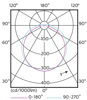
Light Distribution Diagram - LED PLC 6.5W 865 2P G24d-2
