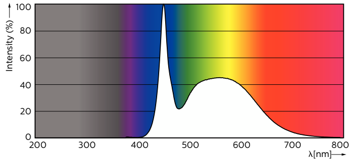
Spectral Power Distribution Colour - LED PLC 6.5W 865 2P G24d-2
