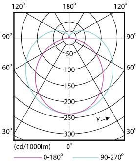
Light Distribution Diagram - MAS LEDtube 1200mm HO 16W840 T8 RN
