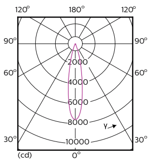
PAR38 120V 17-120W 25D 3000K E26 D BL
