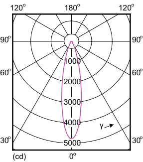
Light Distribution Diagram - 16PAR38/AMB/F25/827/DIM ULW
