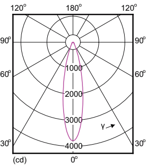
Light Distribution Diagram - 13.5PAR38/AMB/F25/827/DIM ULW
