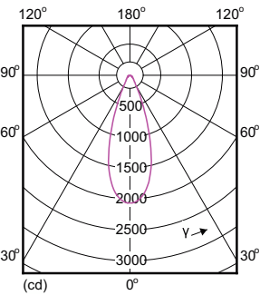
Light Distribution Diagram - 13.5PAR38/AMB/F40/827/DIM ULW
