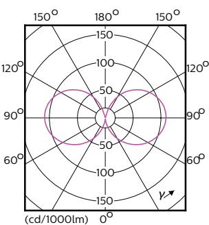
Light Distribution Diagram - TForce LED HPL ND 32-25W E27 740 CL
