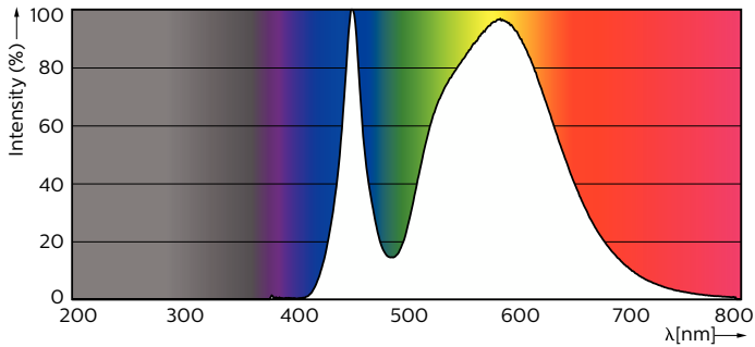
Spectral Power Distribution Colour - TForce LED HPL ND 29-25W E27 740 FR
