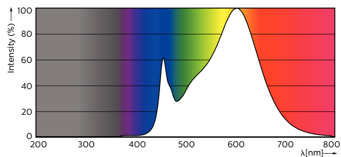
Spectral Power Distribution Colour - MAS LEDtube 1200mm UO 16W 830 T8
