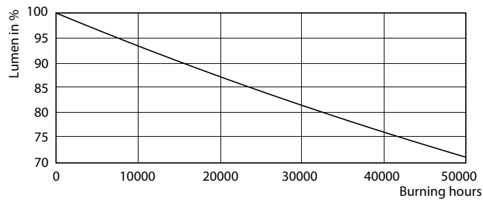
Lumen Maintenance Diagram - MAS LEDtube 1200mm UO 16W 840 T8
