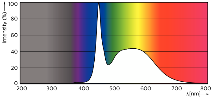
Spectral Power Distribution Colour - MAS LEDtube 1200mm UO 16W 865 T8
