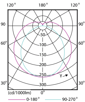
Light Distribution Diagram - MAS LEDtube 1500mm UO 24W 830 T8
