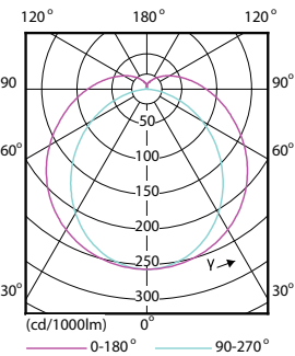
Light Distribution Diagram - MAS LEDtube 1500mm HO 20W840 T8
