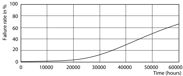
Life Expectancy Diagram - MAS LEDtube 1500mm HO 20W865 T8
